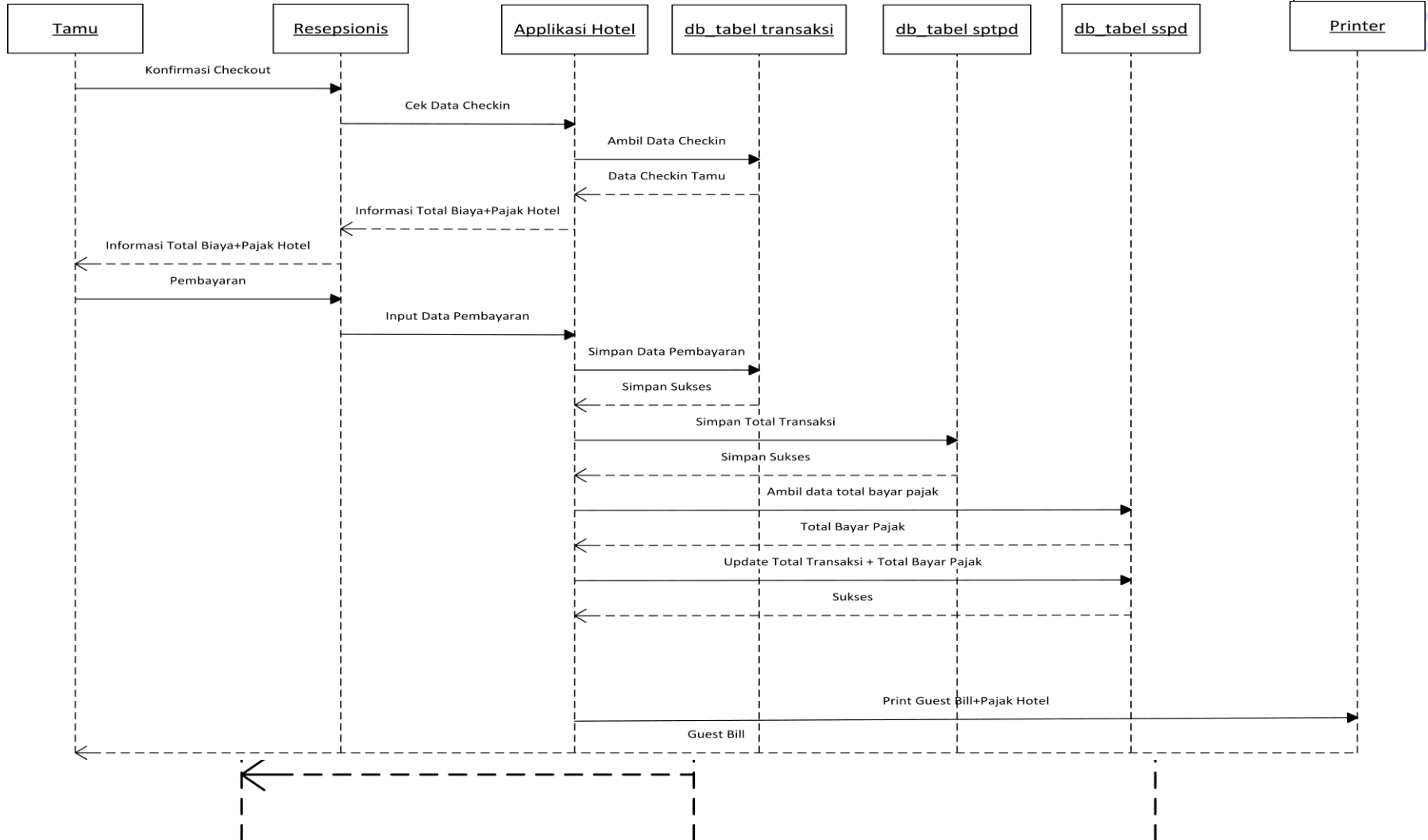
Sequence Diagram Proses Transaksi Hotel
